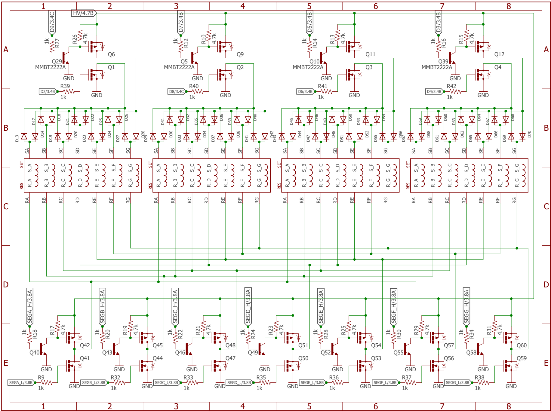
Coyt Barringer Segment Driving and Multiplexing Section
